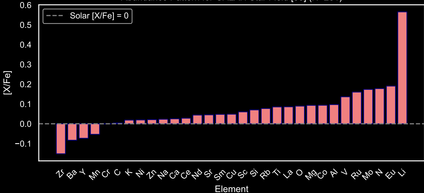
Abundance Pattern for GALAH Star Field [33] (N=281)
