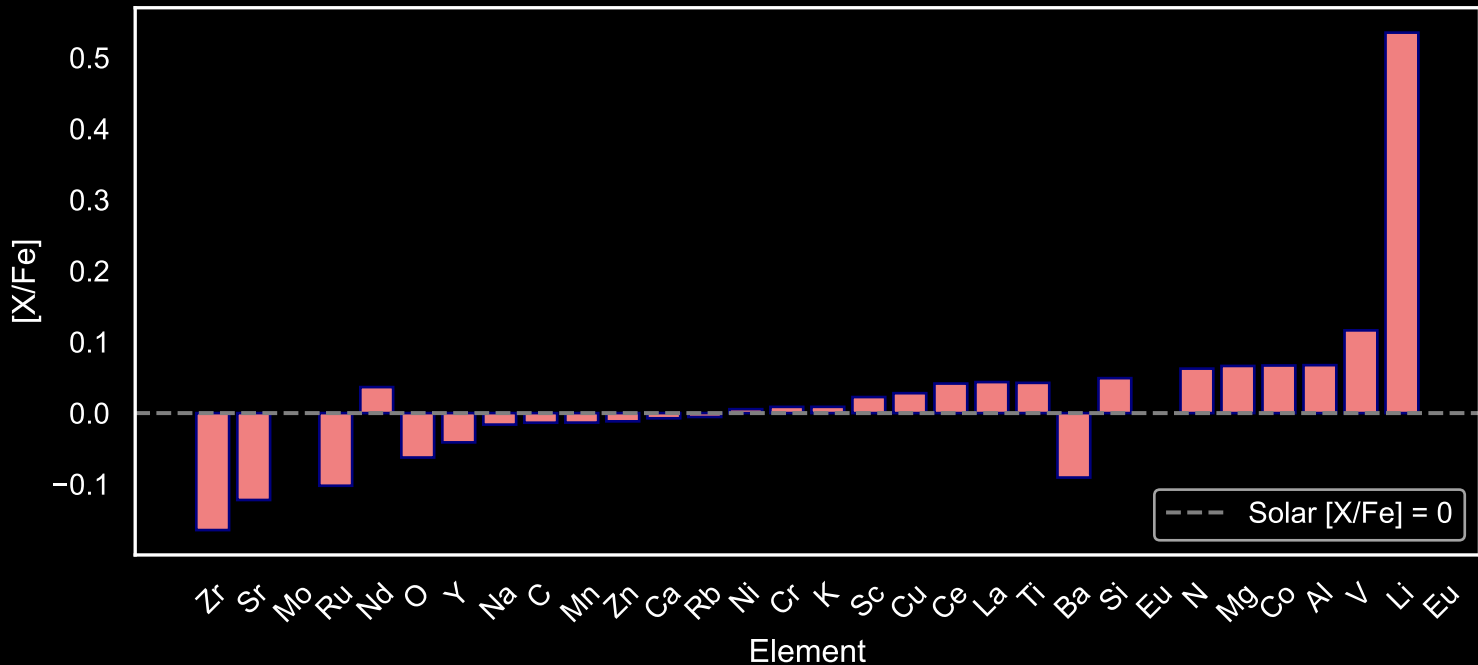
Abundance Pattern for GALAH Main Sequence Stars: Star Field [33] (N=135)
