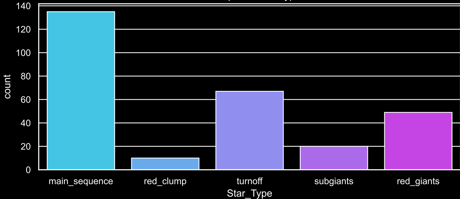
Field [33] Count plot of Star Type
