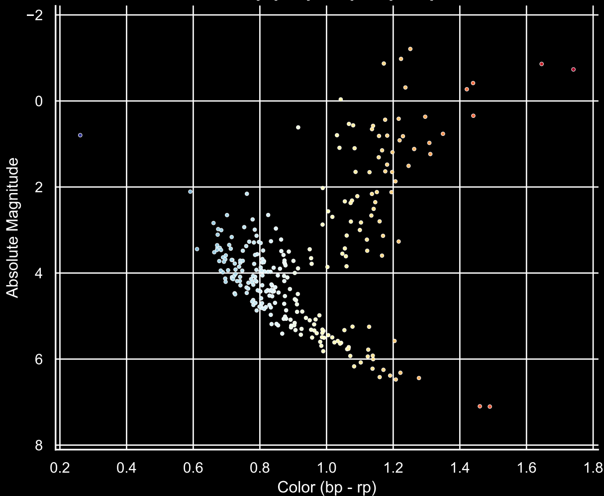
GALAH Hertzsprung-Russell Diagram Field [33] Ra [342.35] Dec [-67.08]
