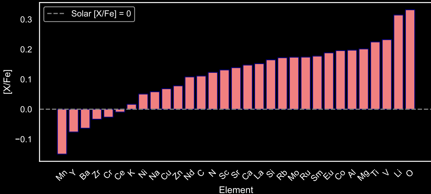
Abundance Pattern for GALAH Red Giants: Star Field [33] (N=59)
